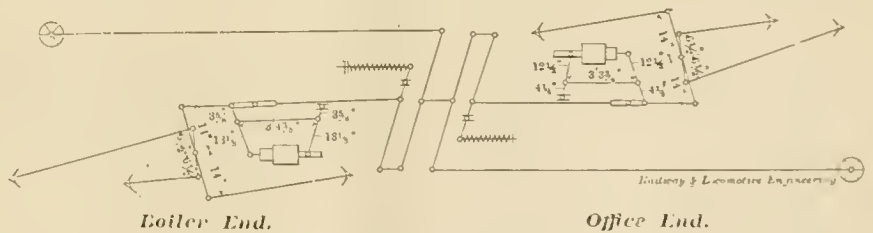
LEVERAGE OF DIVIDED OR TWIN BRAKE.
